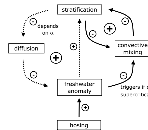
Figure 5: Schematic of the two interacting feedbacks.
