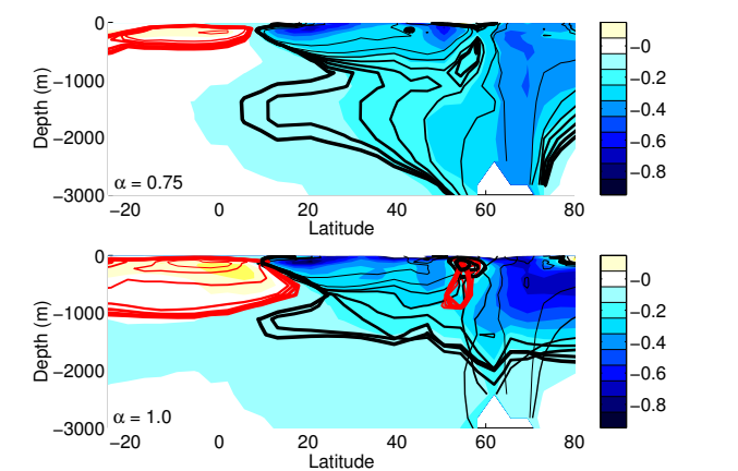
Figure 4: Temporal evolution of the zonally averaged temperature and salinity anomalies. Upper panel: \alpha = 0.75 , lower panel: \alpha = 1 . Background shading: Salinity anomaly in PSU after 300 years of 0.1 Sv anomalous freshwater flux. Black lines: Position of the zonally averaged -0.2 PSU salinity anomaly, starting at t = 100 years with the thinnest line, line thickness increasing with 50 years time steps. Thickest line shows the position at t = 450 years. Red lines: the same as black, but for the zonally averaged 0.7 K temperature anomaly. The values of the contours were chosen such that they represent approximately the same change in density.
