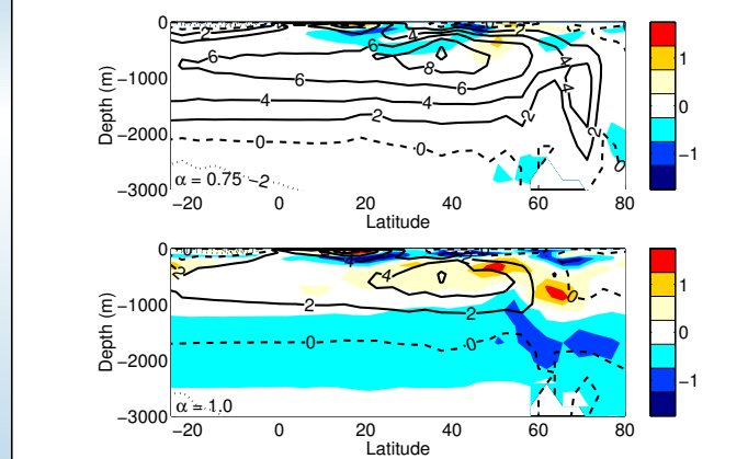
Figure 6: Changes in mixing and overturning after 800 years of 0.1 Sv freshwater flux. Shading: zonally averaged anomalies of the background diffusivity \kappa in 10^{-6} \text{ m}^2 \text{ s}^{-1} . Contours: overturning streamfunction in Sv. Upper panel: \alpha = 0.75 , lower panel: \alpha = 1 . A layer of lower diffusivity is formed by the freshwater anomaly in the supercritical case (lower panel). The freshwater confined to the upper ocean by this layer inhibits deep convection. In the subcritical case (upper panel), diffusivity anomalies are small.
