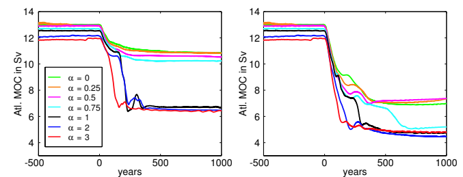
Figure 2: The maximum of the Atlantic Meridional Overturning. Left: sfx01 runs, right: sfx02 runs. The anomalous freshwater forcing is started at t = 0 . In both the sfx01 and sfx02 runs, there are two distinct groups of experiments, separated by a critical value \alpha_{cr} .
