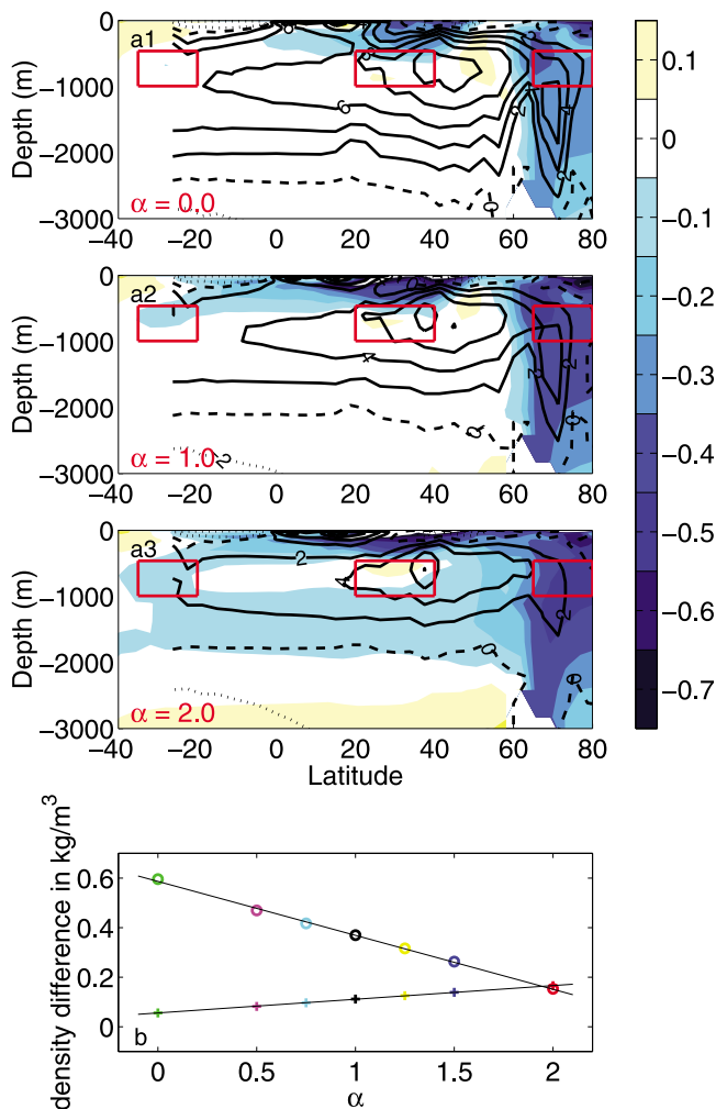
Figure 3. (a) Shading: zonally averaged Atlantic density anomalies at 0.25 Sv freshwater forcing of the increasing branch in \text{kg m}^{-3} . Contours: Atlantic overturning stream function at the same freshwater forcing, solid: positive, dashed: zero contour, dotted: negative. Contour spacing is 2 Sv. Red boxes indicate the areas between which the density difference in Figure 3b were calculated. (b) density difference in the Atlantic between the areas 65°N to 80°N and 20°N to 40°N (circles), and between 20°N to 40°N and 20°S to 35°S (crosses), averaged between 460 m and 1000 m depth (red boxes in Figure 1a), as a function of \alpha , at 0.25 Sv freshwater forcing. Colors as in Figure 1a.
