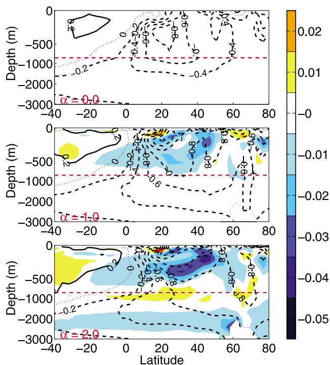
Figure 2. Shading: zonally averaged Atlantic vertical diffusivity anomalies at 0.25 Sv freshwater forcing of the increasing branch in \text{cm}^2 \text{s}^{-1} . Contours: zonally averaged Atlantic salinity anomalies at the freshwater forcing, solid: positive, dotted: zero contour, dashed: negative. Contour spacing is 0.2 psu. Note that the vertical axis above 700 m depth (red dashed line) is stretched; 700 m is approximately the level of no motion. (top) \alpha = 0 , (middle) \alpha = 1 , and (bottom) \alpha = 2 .
