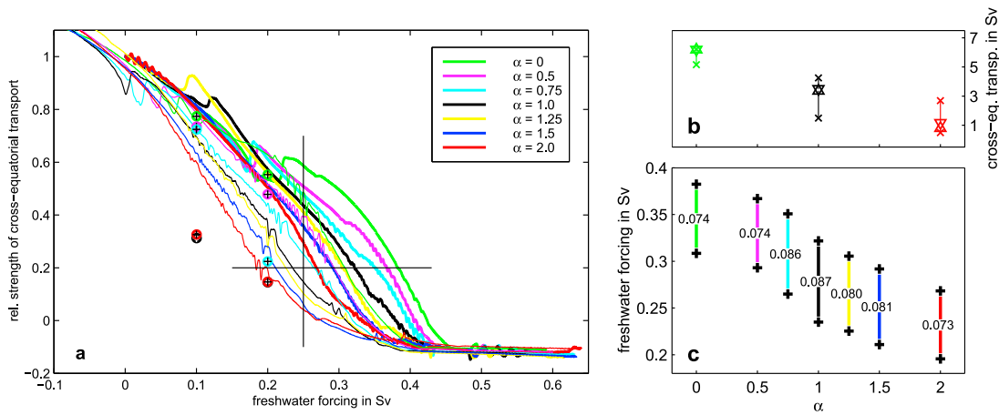
Figure 1. (a) Relative strength of the cross-equatorial volume transport as a function of the freshwater forcing, thick lines: increasing freshwater forcing, thin lines: decreasing freshwater forcing. Circles with black crosses: reference values from the experiments with abruptly increased freshwater forcing from Marzeion et al. [2007]. Black lines indicate the freshwater forcing and overturning strength at which the values in Figures 1b and 1c, and Figures 2 and 3 were taken. (b) Cross-equatorial transport as a function of \alpha at 0.25 Sv of freshwater forcing. Crosses indicate the transport during the transient increase and decrease of the freshwater forcing. Downward (upward) pointing triangles indicate the transport after 2000 yrs of constant freshwater forcing, branching off the increasing (decreasing) branch of the freshwater forcing. (c) Strength of the freshwater forcing at which the cross-equatorial transport is 20% of the unperturbed state, as a function of \alpha ; upper values for the branch of increasing freshwater forcing, lower values for the branch of decreasing freshwater forcing; the numbers indicate the difference between the two values.
