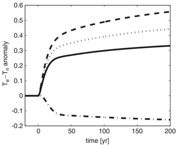
Fig. 6. Anomaly of the temperature difference between low latitudes and northern box. Dashed, dotted, solid as in Figs. 2 and 5, dash-dotted for \alpha = 3 .
