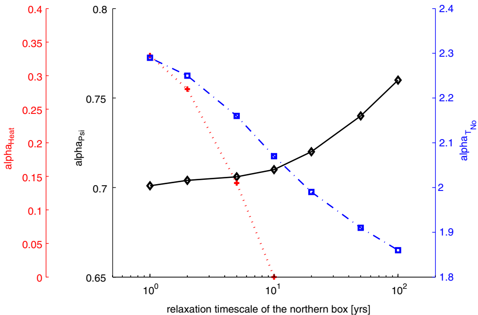
Fig. 7. Dependency of the critical values of \alpha on the timescale of temperature relaxation in the northern box. Dotted line: \alpha_{Heat} , dash-dotted line: \alpha_{T_{No}} , solid line: \alpha_{Psi} .
