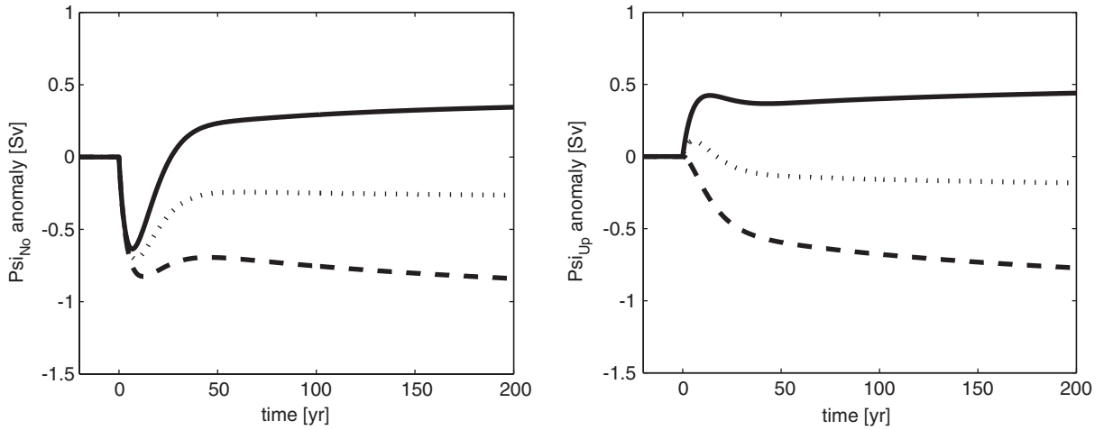
Fig. 5. As Fig. 2, but left: anomalous northward volume transport. Right: upwelling into the thermocline box.
