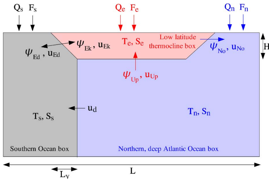
Fig. 1. Schematic representation of the model.
